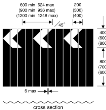
515.1A Sharp deviation of route at a roundabout
