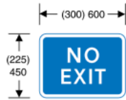
835 Exit from a car park, private access road or property to a public road not allowed
