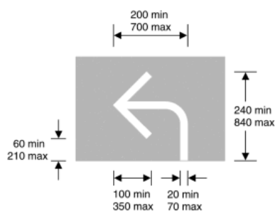
6003 Vehicular traffic must leave at next junction
