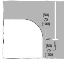
1026.1 Part of the carriageway outside an entrance to off-street premises or a private drive, or where the kerb is dropped to provide a convenient crossing place for pedestrians, which should be kept clear of waiting vehicles
