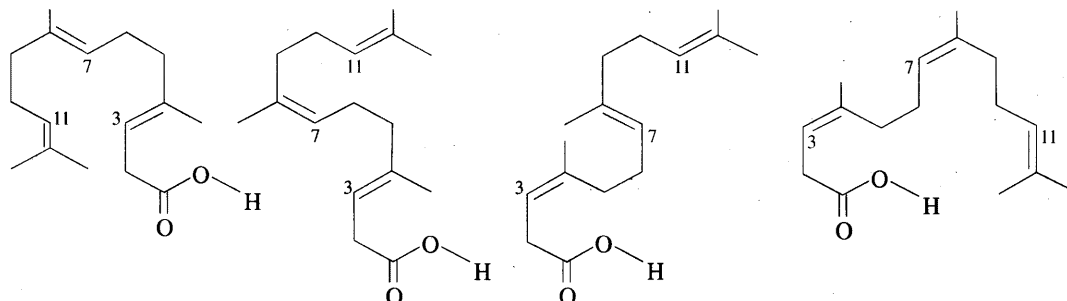
3,7-trans/trans- isomer
