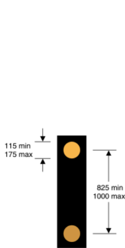
6023 Light signal conveying the warning prescribed in regulation 45
