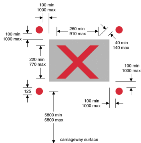
6031.1 Light signals conveying the requirement prescribed in regulation 38(b)
